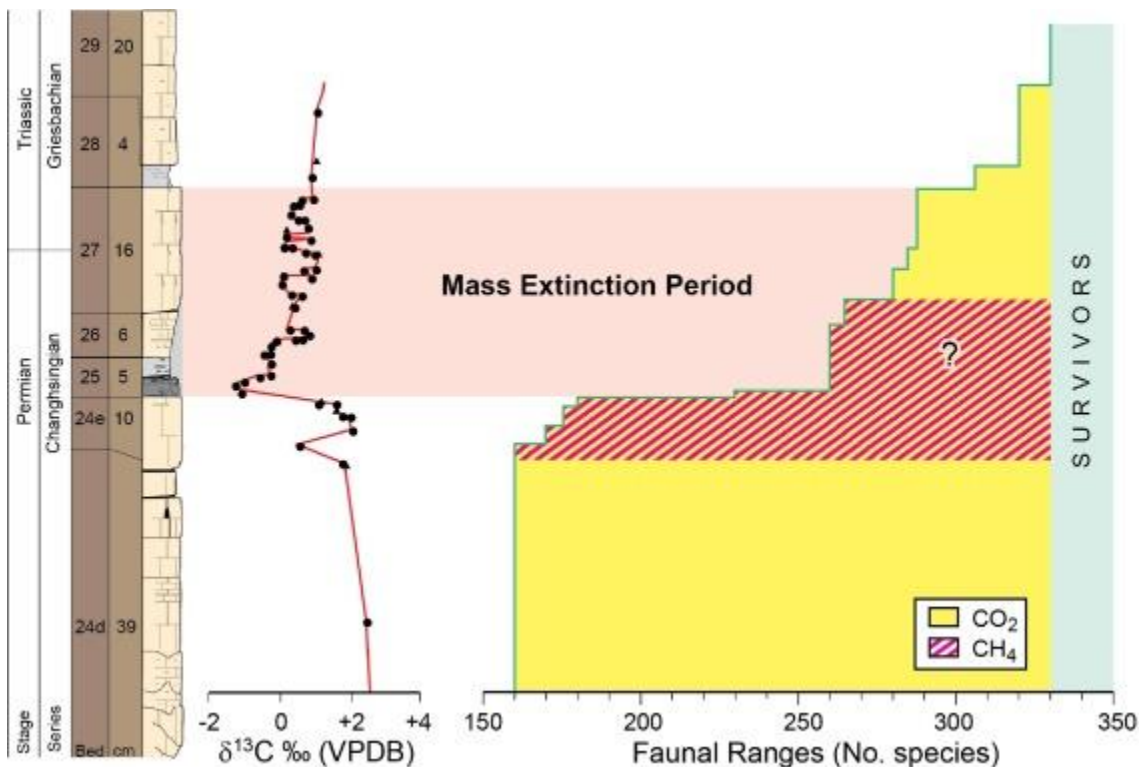
Fig. 1. \delta^{13}\text{C} excursion, faunal disappearances and gas compositions about the end Permian (GSSP section at Meishan, China). Atmospheric greenhouse gas was dominated by CO 2 prior to the event with a sudden surge in CH 4 during the latest stage leading into the event. Stratigraphy of Meishan section is from Yin et al. (2001) , whereas faunal decline and carbon isotope trend are from Jin et al. (2000) , and duration of the mass extinction period is from Burgess et al. (2014) .
